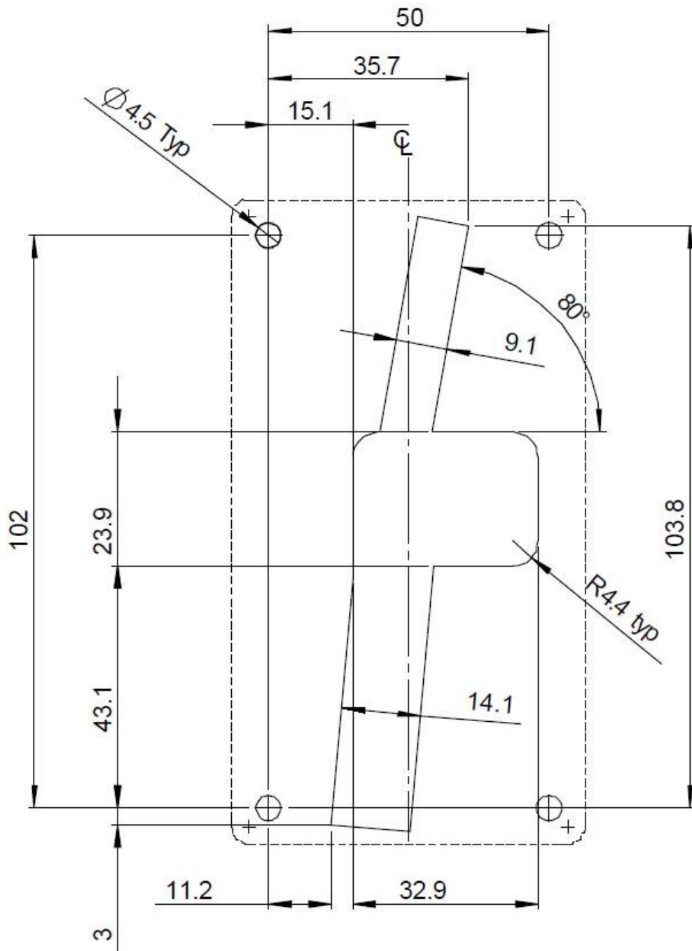
VIEW FROM REAR OF PANEL
