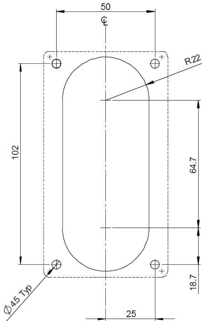
VIEW FROM FRONT OF PANEL
